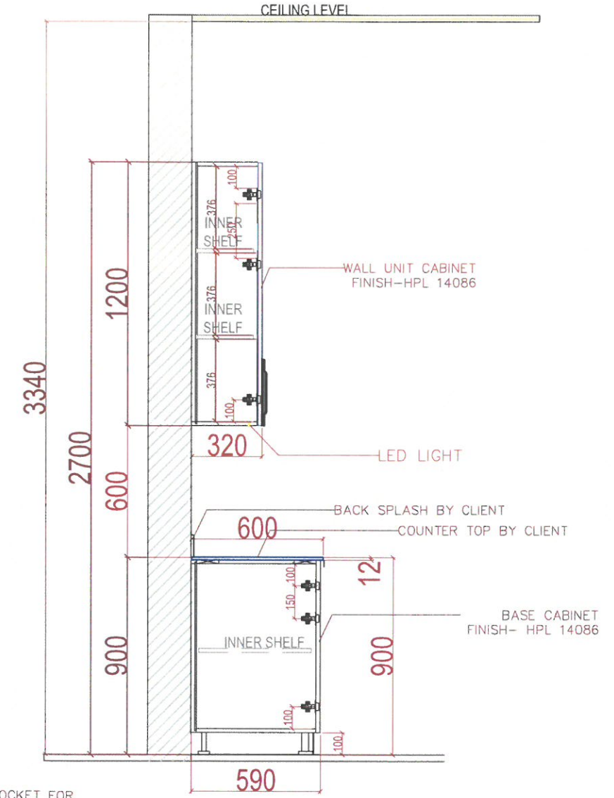
SECTION-
