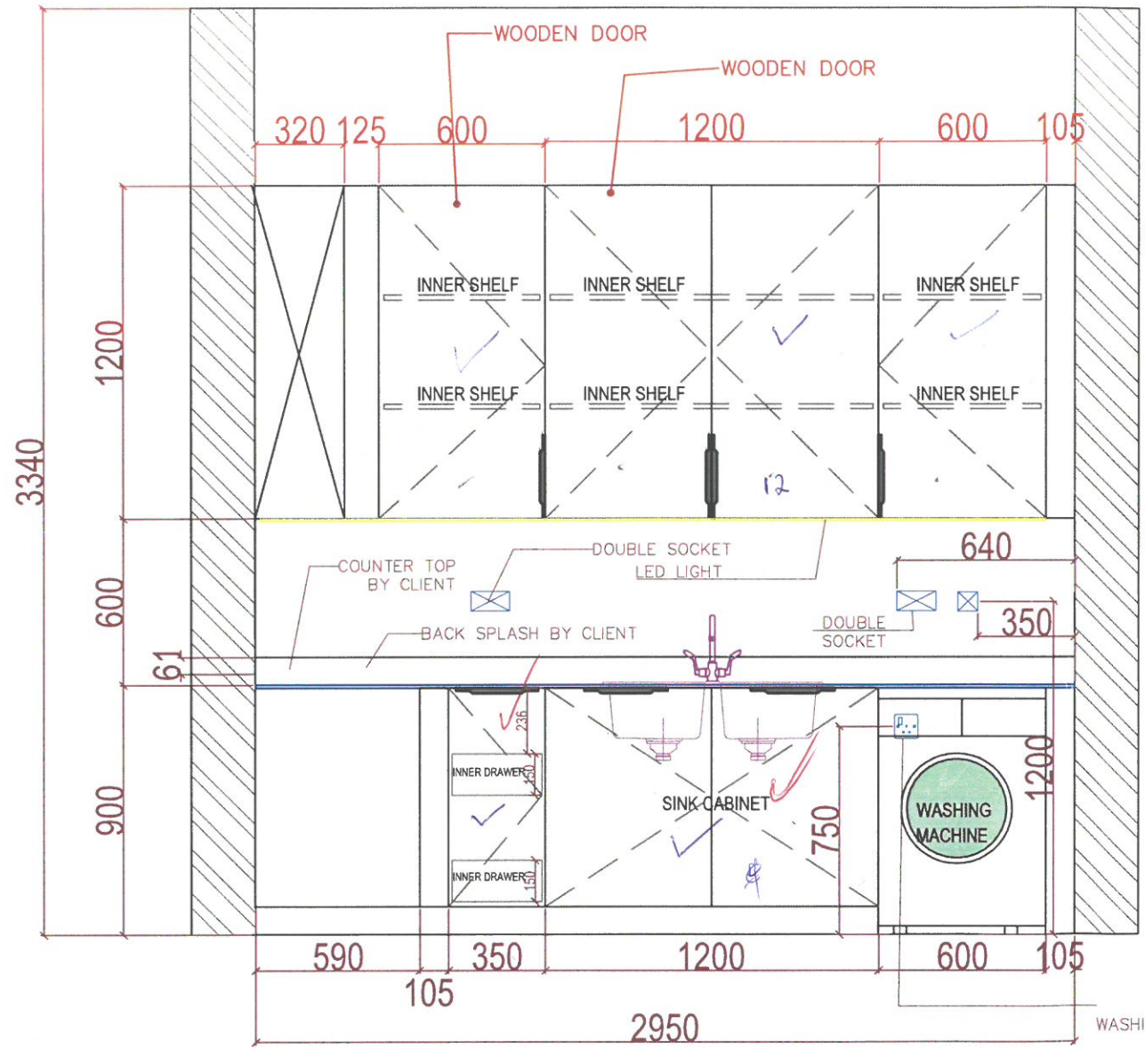
ELEVATION -C
